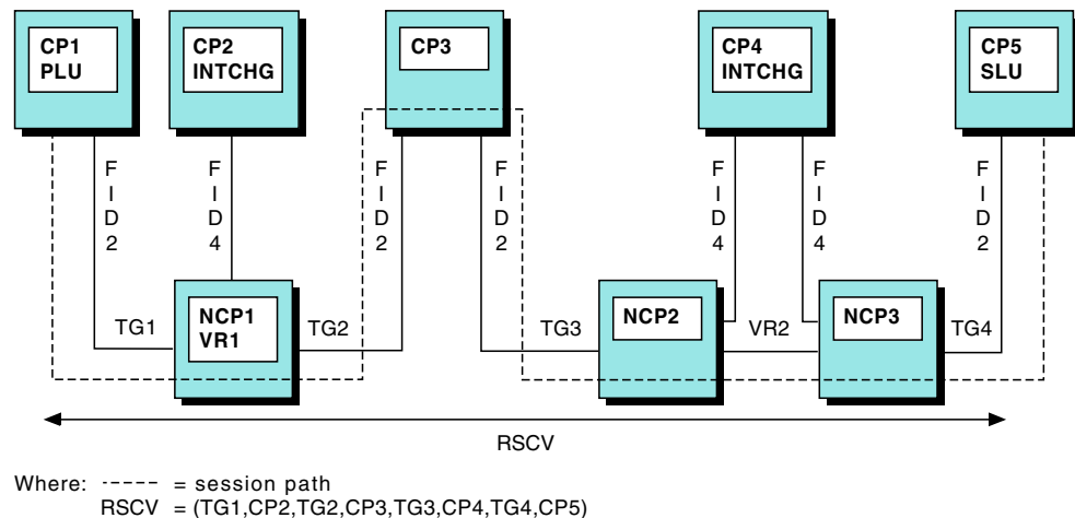
Figure 235. SNA Advanced Peer-to-Peer Networking Session through Nonadjacent Composite Nodes
