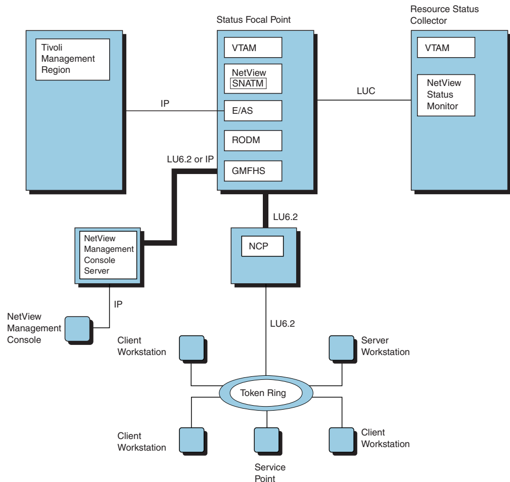
Figure 15. Host-to-Workstation Connection
