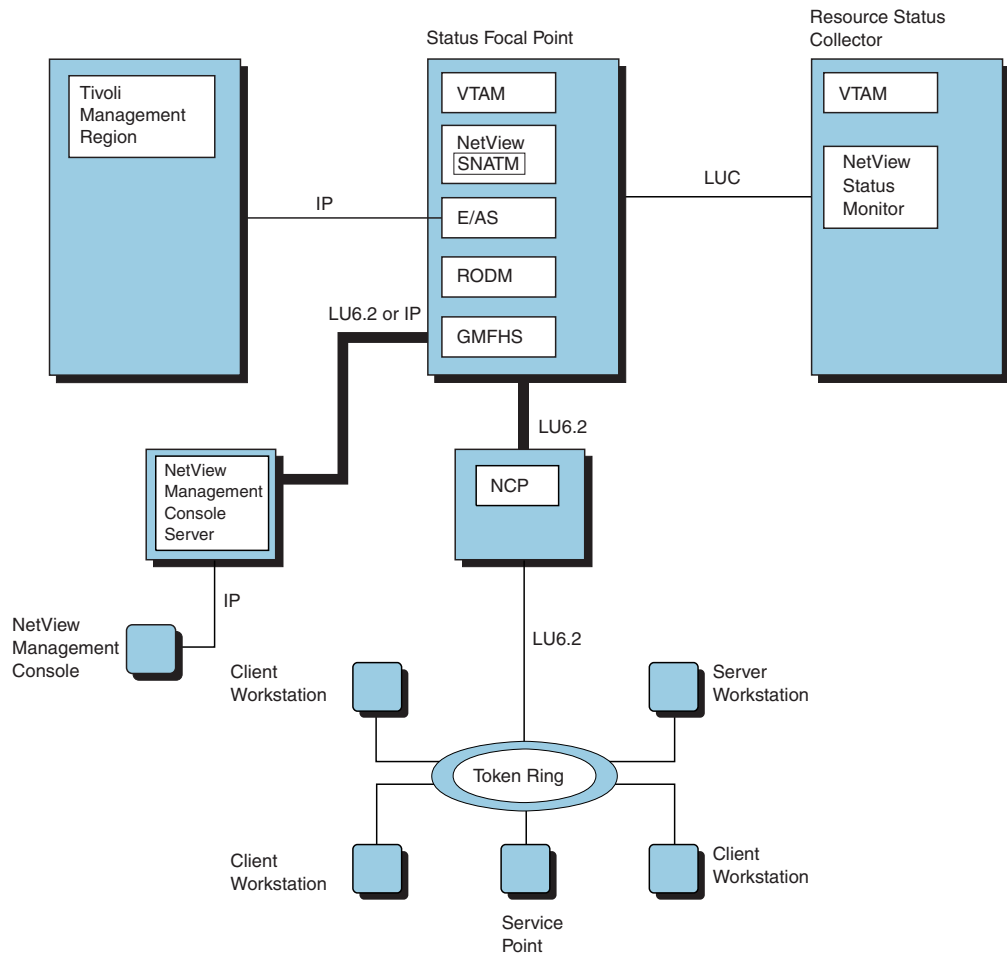
Figure 245. Network Management Structure
