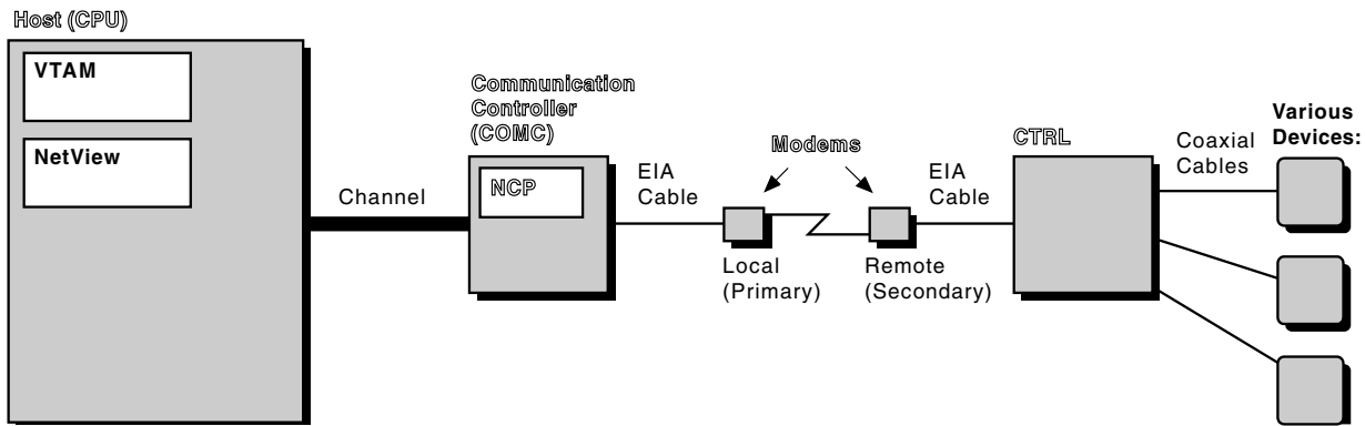
Figure 229. Hardware Monitor Physical Components and Levels
