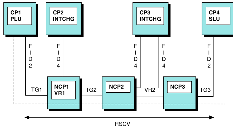
Figure 236. SNA Advanced Peer-to-Peer Networking Session through Adjacent Composite Nodes with FID2 Connection
