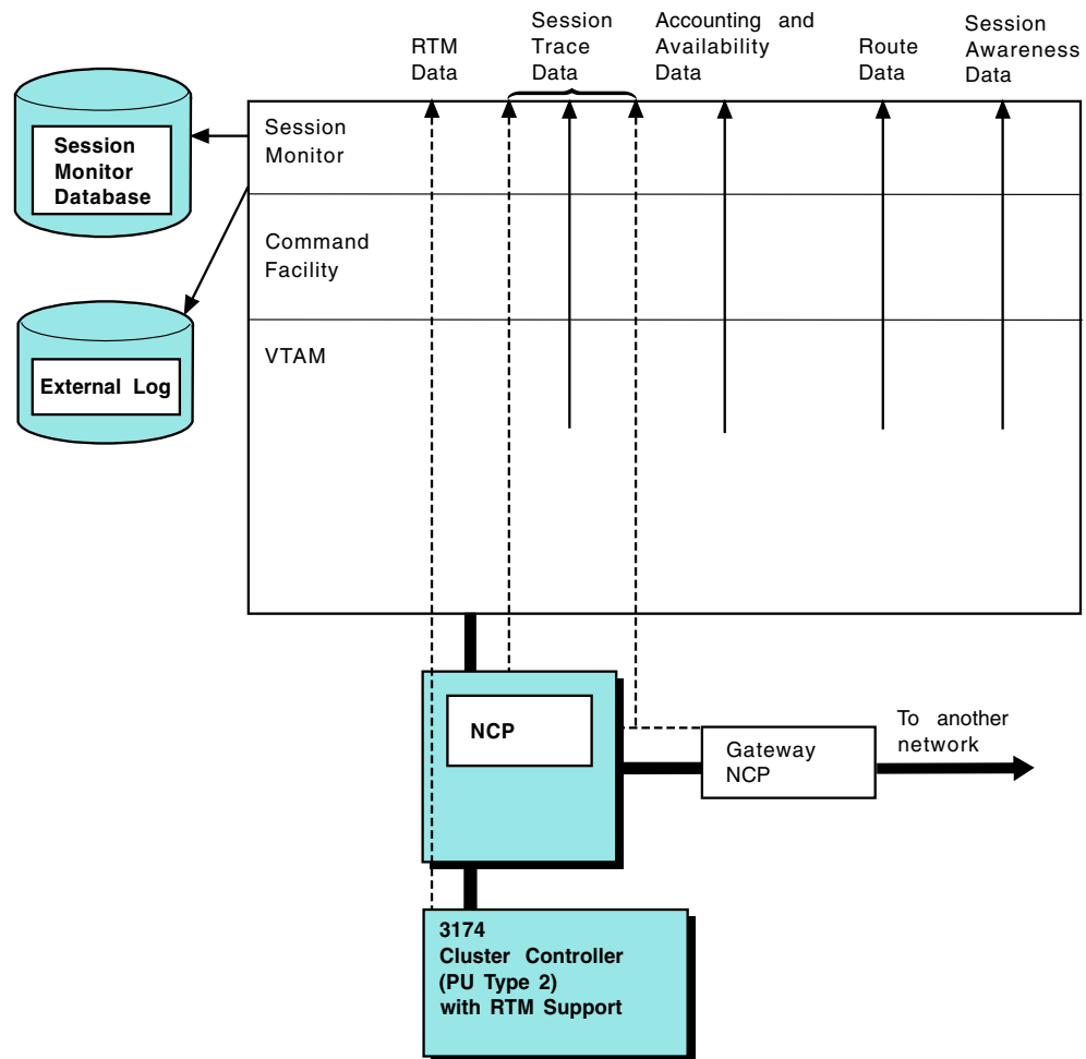
Figure 57. Session Monitor Data Collection
