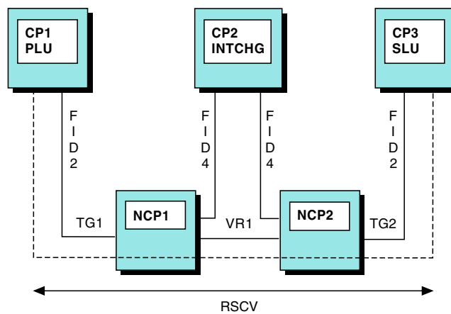
Figure 234. SNA Advanced Peer-to-Peer Networking Sessions through Composite Nodes
