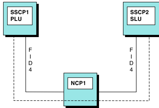
Figure 233. SNA Session
