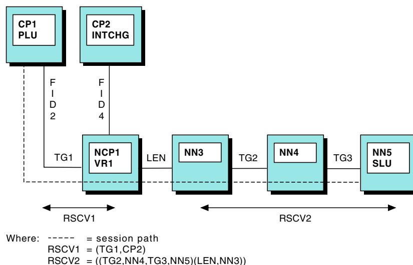
Figure 239. Session between 2 SNA Advanced Peer-to-Peer Networking Subnetworks through a LEN Connection
