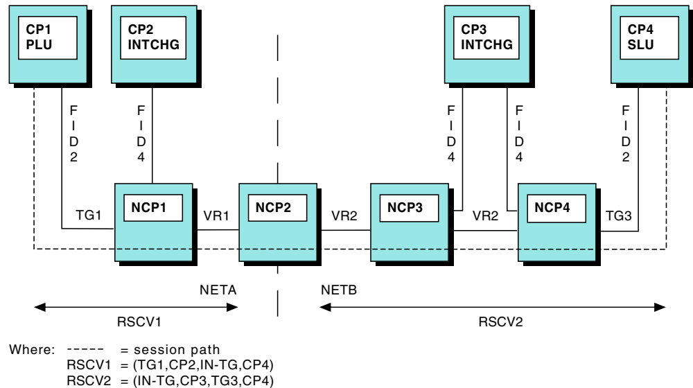
Figure 238. SNA Advanced Peer-to-Peer Networking Session through SNI Gateway
